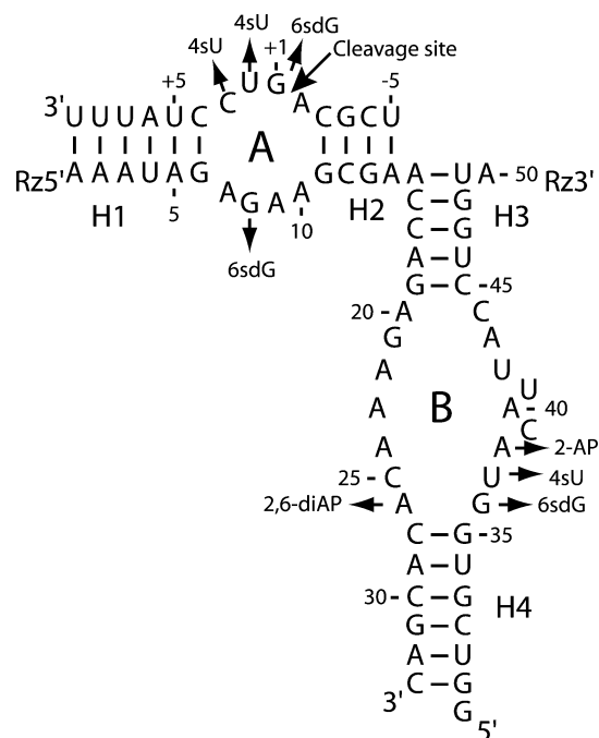
FIGURE 1: The hairpin ribozyme–substrate complex. The secondary structure of the hairpin ribozyme complex used in this study includes modifications in helices 1 and 2 in the substrate and the ribozyme 5' strand as well as a rate-enhancing U39C mutation in the ribozyme 3' strand. Domains A and B and helices 1–4 are indicated. The cleavage site is shown by an arrow. Nucleotides at positions +1, +2, +3, 8, 26, 36, 37, and 38 were individually substituted by modified nucleotides, i.e., 4-thiouridine (4sU), 6-thiideoxyguanosine (6sdG), 2,6-diaminopurine (2,6diAP), or 2-aminopurine (2-AP) as indicated by small arrows.
