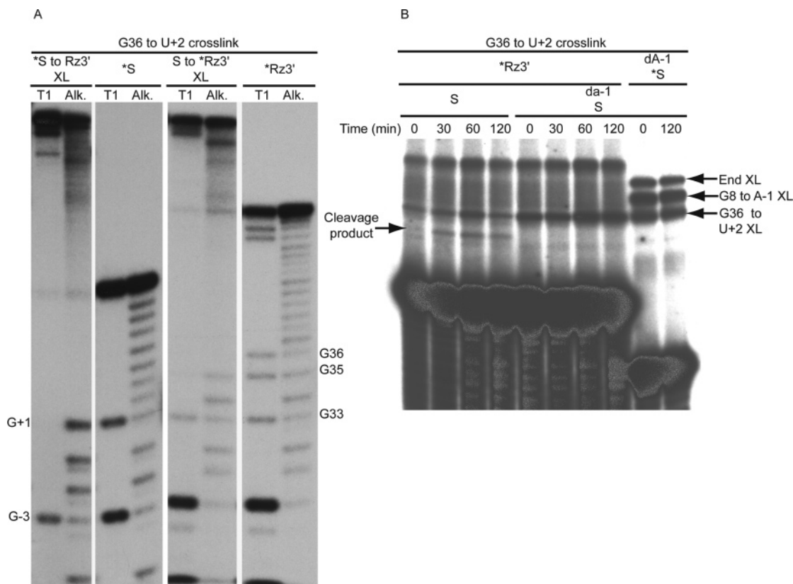
FIGURE 2: G36/U+2 cobalt hexaammine-induced crosslinks. (A) Mapping of G36/U+2 cobalt hexaammine-induced crosslink. The crosslinked sites were mapped by limited alkaline hydrolysis (Alk) and partial digestion with RNase T1 (T1). The species consisting of the 5'- 32 P end-labeled substrate crosslinked to the ribozyme 3' strand (*S to Rz3' XL) and the end-labeled substrate control (*S) are paired on the left. The species consisting of the 5'- 32 P end-labeled ribozyme 3' strand crosslinked to substrate (S to *Rz3' XL) and the end-labeled ribozyme 3' strand control (*Rz3') are paired on the right. Sites of T1-induced cleavages are indicated by the numbered guanosine (note that the G+1 band appears in the alkali track but is poorly cleaved by T1 RNase because of its proximity to the branched crosslink structure). (B) Cleavage assay with the crosslinked end-labeled ribozyme 3' strand crosslinked to cleavable or noncleavable (2'-deoxyA-1) substrate. Since the ribozyme 3' strand is crosslinked to residue U+2, cleavage removes the 5' cleavage product (5 nt) from the crosslinked species, generating a band with slightly increased mobility. Crosslinks were generated as described in Materials and Methods and then simply incubated to permit cleavage. Crosslinks made with end-labeled noncleavable substrate (at right) identify the crosslinked species.
