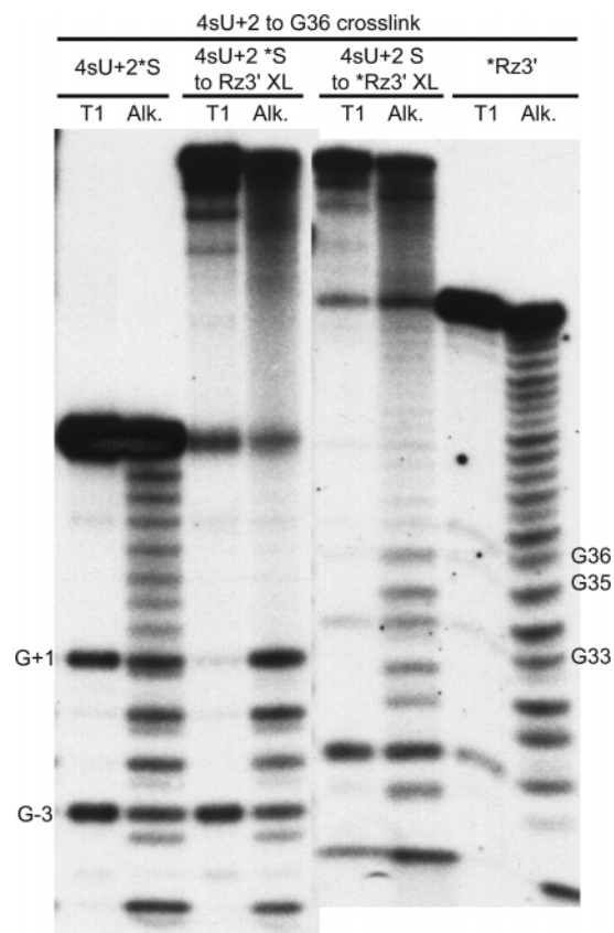
FIGURE 3: Mapping of 4sU+2/G36 crosslinked sites. The crosslinked sites were mapped by limited alkaline hydrolysis (Alk) and partial digestion with RNase T1 (T1). The species consisting of the 5'- 32 P end-labeled 4sU+2 substrate crosslinked to the ribozyme 3' strand (4sU+2*S to Rz3' XL) and the end-labeled 4sU+2 substrate control (4sU+2*S) are paired on the left. The 5'- 32 P end-labeled ribozyme 3' strand crosslinked to the 4sU+2 substrate (4sU+2S to *Rz3' XL) and the end-labeled ribozyme 3' strand control (*Rz3') are paired on the right. Sites of T1-induced cleavages are indicated by the numbered guanines.
