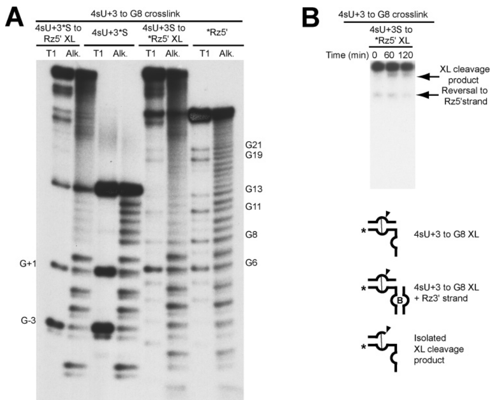
FIGURE 5: 4sU+3 crosslink. (A) Mapping of 4sU+3 crosslinked sites. The crosslinked sites were mapped by limited alkaline hydrolysis (Alk) and partial digestion with RNase T1 (T1). The species consisting of the 5'- 32 P end-labeled 4sU+3 substrate crosslinked to the ribozyme 5' strand (4sU+3*S to Rz5' XL) and the end-labeled 4sU+3 substrate control (4sU+3*S) are paired on the left. The species consisting of the 5'- 32 P end-labeled ribozyme 5' strand crosslinked to the 4sU+3 substrate (4sU+3S to *Rz5' XL) and the end-labeled ribozyme 5' strand control (*Rz5') are paired on the right. Sites of T1-induced cleavages are indicated by the numbered guanosine. (B) Activity assay for isolated crosslinked species. The ribozyme 3' strand (Rz3') was added to crosslinked products, labeled on the ribozyme 5' strand as indicated, in the presence of 1 mM cobalt hexaammine for up to 2 h. The crosslink cleavage product and the reversal to the ribozyme 5' strand are shown by arrows.
