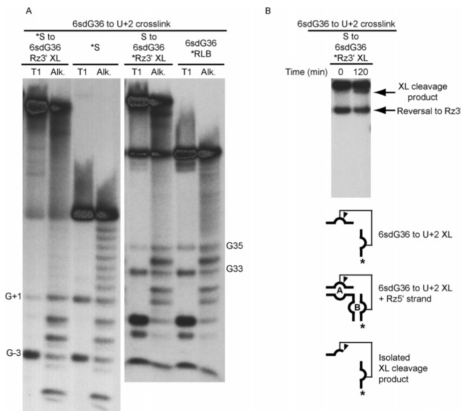
FIGURE 4: 6sdG36 crosslink. (A) Mapping of 6sdG36 crosslinked sites. The crosslinked sites were mapped by limited alkaline hydrolysis (Alk) and partial digestion with RNase T1 (T1). The species consisting of the 5'- 32 P end-labeled substrate crosslinked to the 6sdG36 ribozyme 3' strand (*S to 6sdG36Rz3' XL) and the end-labeled substrate control (*S) are paired on the left. The species consisting of the 5'- 32 P end-labeled 6sdG36 ribozyme 3' strand crosslinked to substrate (S to 6sdG36*Rz3' XL) and the end-labeled 6sdG36 ribozyme 3' strand control (6sdG36*Rz3') are paired on the right. Sites of ribonuclease T1-induced cleavages are indicated by the numbered guanosine. (B) Activity assay for isolated crosslinked species. The ribozyme 5' strand (Rz5') was added to crosslinked products labeled on the ribozyme 3' strand (*Rz3') in the presence of 1 mM cobalt hexaammine for 2 h. The crosslink cleavage product and the reversal to the ribozyme 5' strand are shown by arrows.
