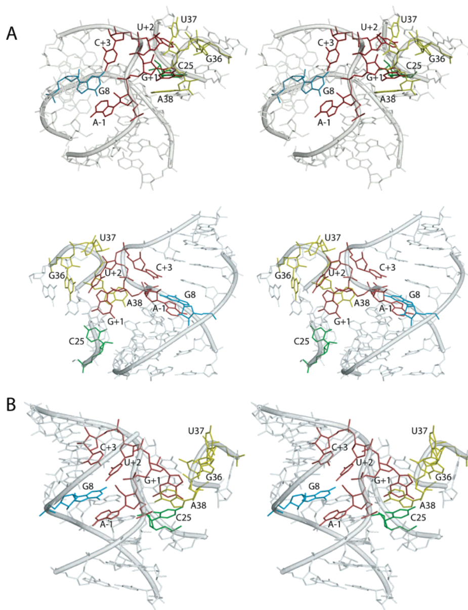
FIGURE 6: Models of the hairpin ribozyme active site. (A) Two different stereoviews of the MC-SYM-generated model based on biochemical and photochemical experiments. Residues A-1, G+1, U+2, and C+3 in the substrate strand are shown in red. G+1 which is stacking on A38 (yellow) and forming a Watson-Crick base pair with C25 (green) in the ribozyme 5' strand is shown. U+2 is bulged out of domain A and is in the vicinity of G36 and U37 (both in yellow) as suggested by crosslinking experiments. Residue C+3 forms a hydrogen bond with A7 and partially stacks on G8 (blue). The latter nucleobase, in the substrate-binding strand, is stacked on A-1, and its Watson-Crick face is adjacent to the scissile bond. Remaining parts of substrate and ribozyme strands are depicted in transparent gray. (B) Stereoview of the crystal structure of the four-way junction hairpin ribozyme catalytic core.
